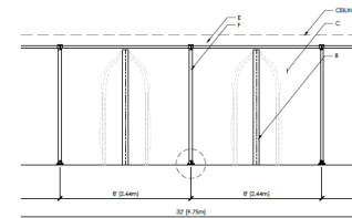
C1 FRONT ELEVATION SCALE: 3/16" = 1'-0"
