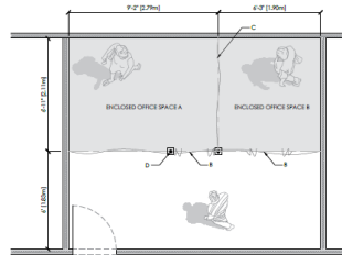
A TYP OFFICE FLOOR PLAN SCALE: 3/16" = 1'-0"
