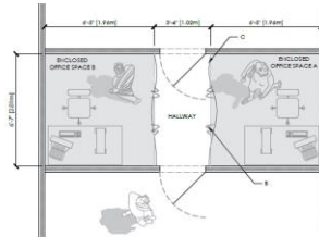
B TYP OFFICE FLOOR PLAN SCALE: 3/16" = 1'-0"
