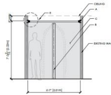
B1 FRONT ELEVATION SCALE: 3/16" = 1'-0"
