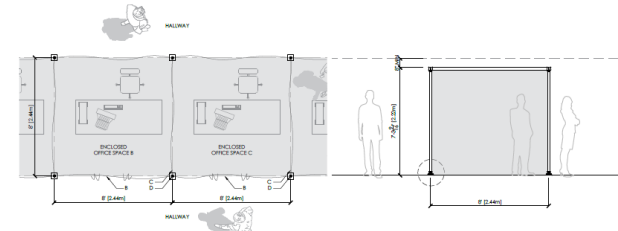
C2 SIDE ELEVATION SCALE: 3/16" = 1'-0"
